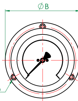
MODEL - 1123 Flush Mounted - Screw Fixing
