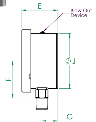
MODEL - 1122 Direct Mounted (Standard)
