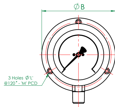
MODEL - 1121 Surface Mounted
