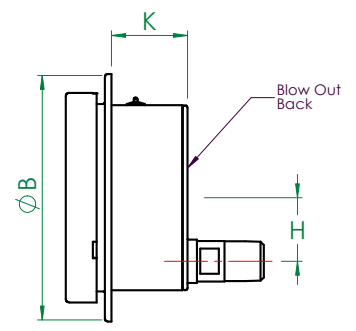
MODEL - 1123 Flush Mounted - Screw Fixing
