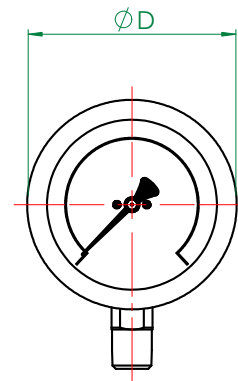
MODEL - 1122 Direct Mounted (Standard)
