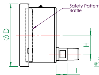
MODEL - 1122BC Direct Mounted (Back Connect)
